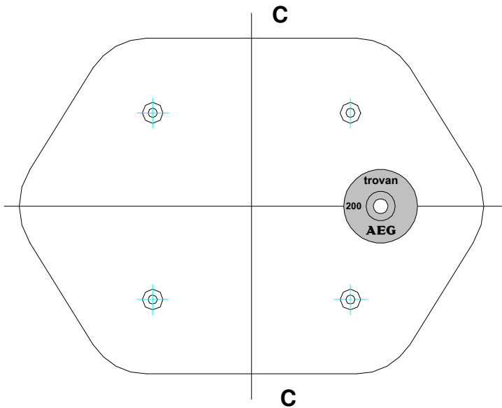
Figure 4.3: Optimal position of the transponder above the antenna (static)
