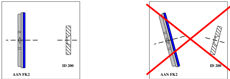
Figure 4.1: Optimal orientation transponder - antenna
