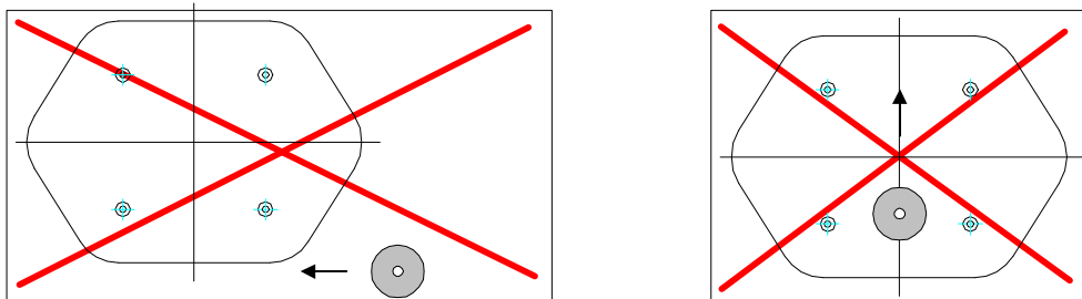
Figure 4.4: Disadvantageous motion paths of the transponder over the antenna
